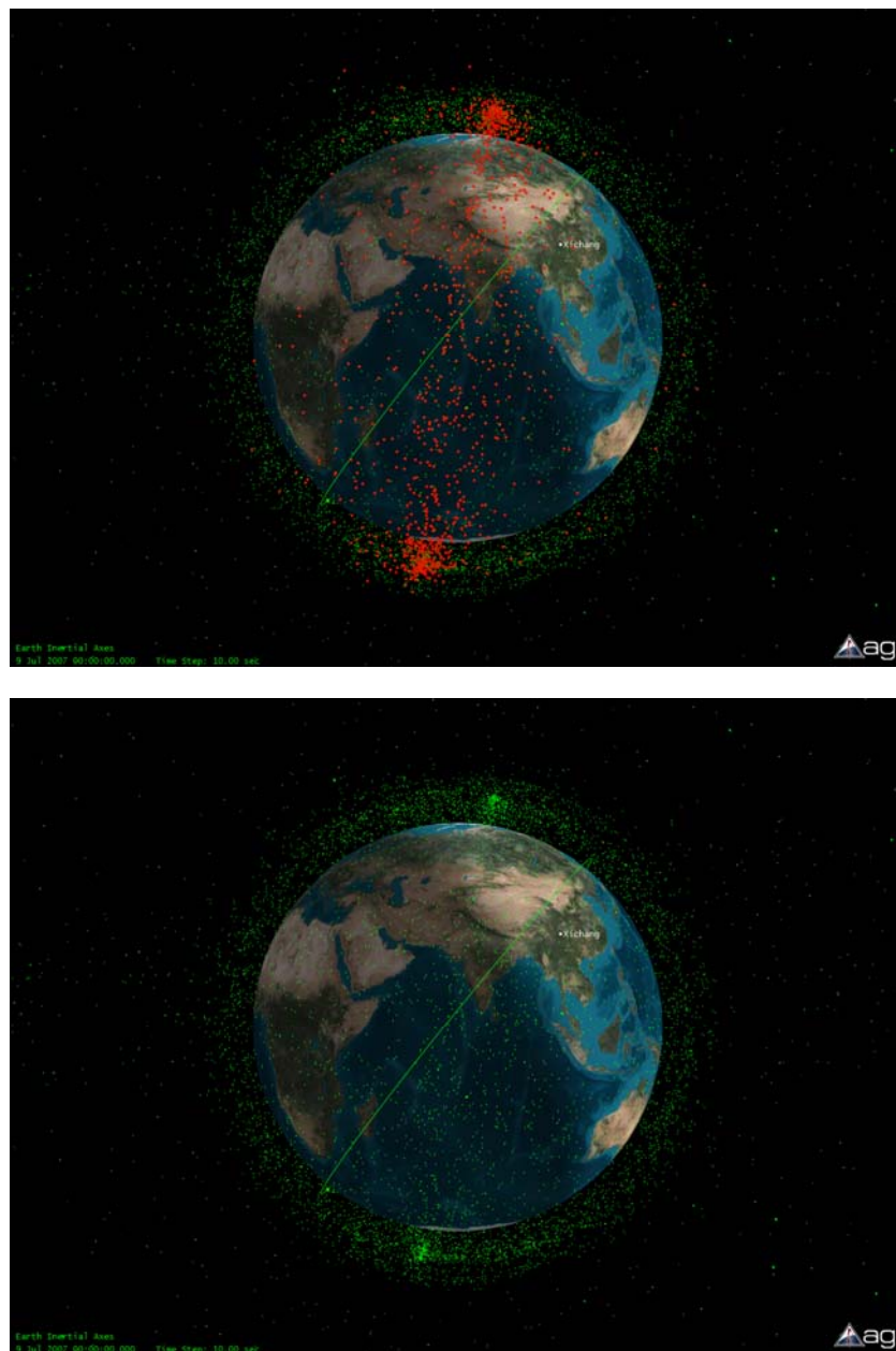
Fig. 9. Distribution of Chinese ASAT Test Debris as of 2007 July 9. Top figure shows the Chinese ASAT Test debris in red, relative to the other debris in Earth orbit. Even without highlighting, the debris cloud is still visible.
