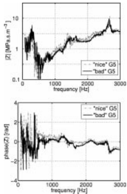
FIG. 8. The impedance spectra of the vocal tract of player A for two configurations associated with a "nice" sound or with a "bad" one, i.e., one which is to be avoided (note G5).
