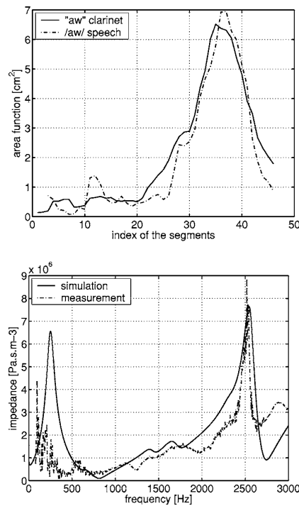
FIG. 11. Top: area function for the vowel /a/ (data from Story and Titze with glottis added). Also shown are the calculated tract configuration named “aw” by clarinetists, as determined from inversion. The abscissa is the element number: the first two are the glottis (see Sec. IV D), the next 44, of length 4 mm comprise a tract 174 mm long. Bottom: the impedance spectrum for the “aw” tract configuration measured on player B.
