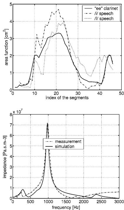
FIG. 10. Top: area function for the vowels /i/ and /u/ (data from Story and Titze with glottis added). Also shown are the calculated tract configuration named “ee” by clarinetists, as determined from inversion. The abscissa is the element number: the first two are the glottis (see Sec. IV D), the next 44, of length 4 mm, comprise a tract 174 mm long. Bottom: the impedance spectrum for the “ee” tract configuration measured on one of the authors (player G) an amateur clarinetist.
