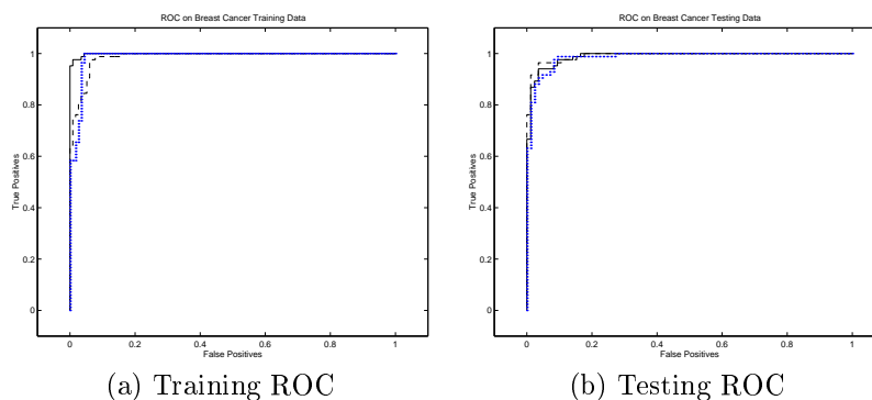
Figure 4: ROC curves on Breast Cancer for discriminative (solid line), Bayes / ML models (dashed line) and SVM linear models (dotted line).
