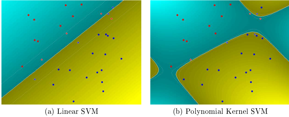
Figure 5: Classification visualization SVMs.
