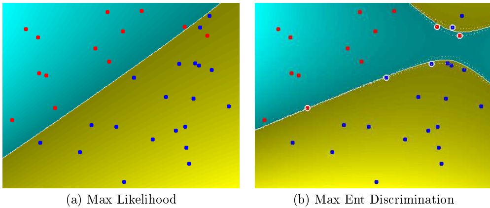
Figure 6: Classification visualization for Gaussian discrimination.
