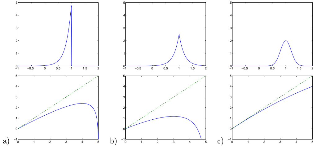
Figure 2: Three margin prior distributions (top row) and the corresponding potential terms (bottom row) from Eq. (15).
