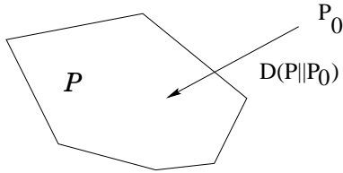
Figure 1: Minimum relative entropy (MRE) projection from the prior distribution to the admissible set.
