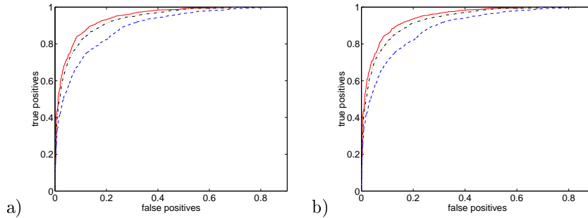
Figure 10: a) test set ROC curves based on a training set with fully labeled examples (solid line), 90% unlabeled and 10% labeled (dot-dashed), only the 10% labeled examples (dashed). In a) a linear kernel was used and in b) a Gaussian kernel.
