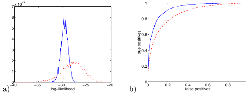
Figure 9: a) Distribution of training set log-likelihoods for the MRE model (solid line) or the Bayes model (dashed-line). b) ROC curve for the two models on an independent test set.
