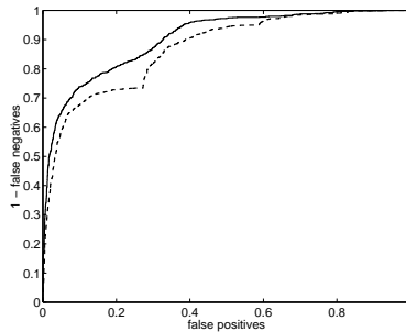
Figure 7: ROC curves for the ME discriminative classifier (full line) and the ML classifier (dashed line) for the splice junction classification problem. The minimum test errors are 12.4% and 14% respectively.
