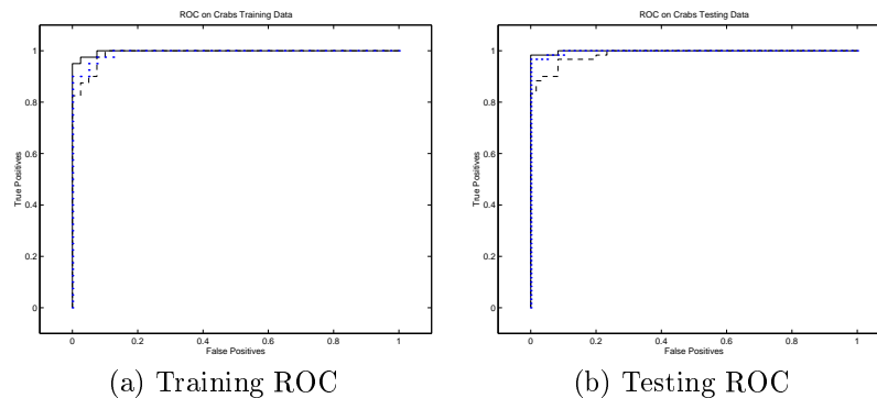
Figure 3: ROC curves on Leptograpsus Crabs for discriminative (solid line), Bayes / ML models (dashed line) and SVM linear models (dotted line).
