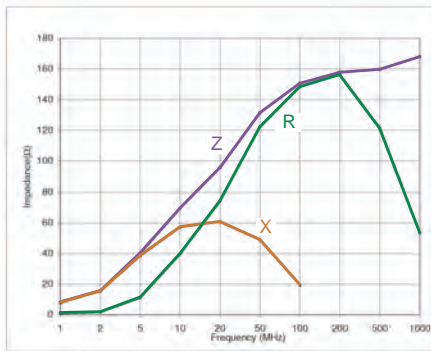
Z-f Characteristics
