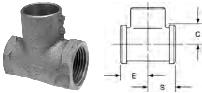
710-3 Tee F x F x C – Cast
