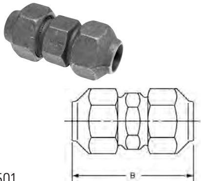
501 Flared Coupling FL x FL – Cast
