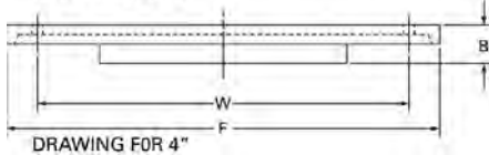
851 DWV Closet Flange C – Cast
