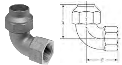
507-3 Flared 90° Elbow FL x F – Cast
