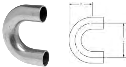
638 Return Bend C x C – Wrot
