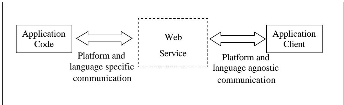
Figure 2.2: SOAP Web-Services Abstraction [SOAP]
