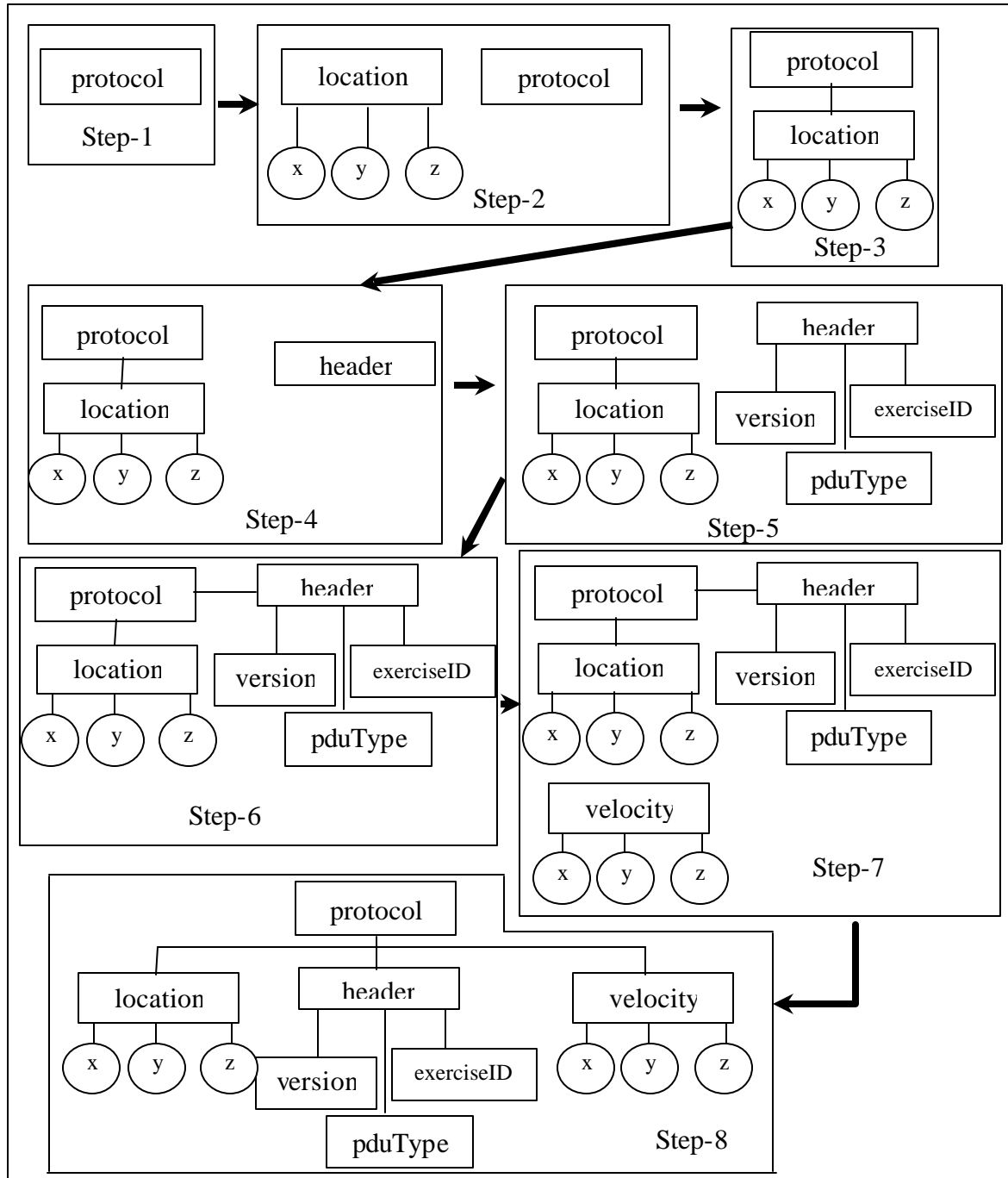
Figure 3.18: XML Deserialization
