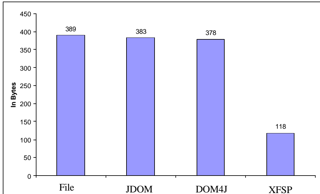
Figure 3.16: Comparison of Serialization Programs
