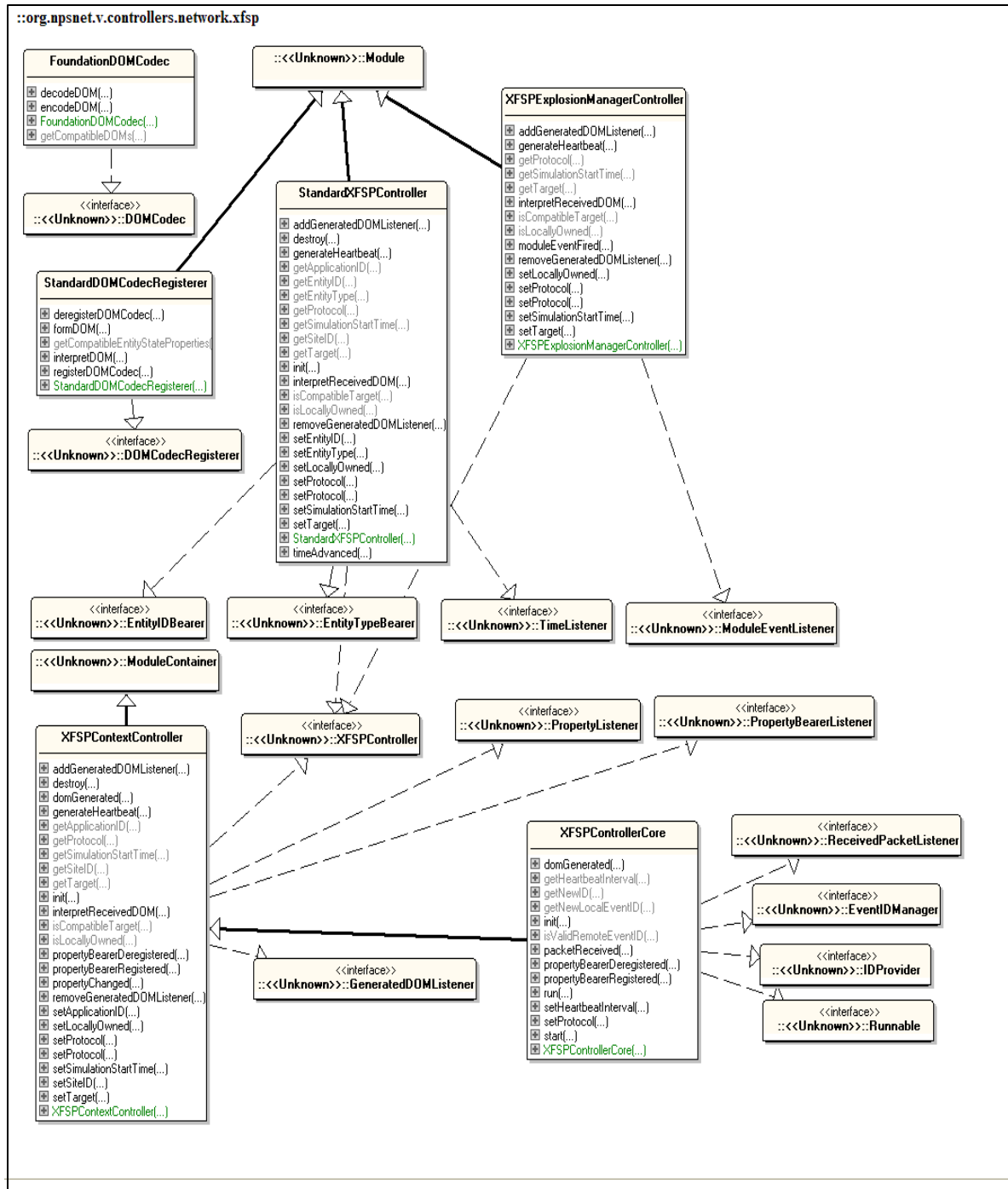
Figure 3.20: StandardXFSPController UML Diagram (Generated by [ESS])
