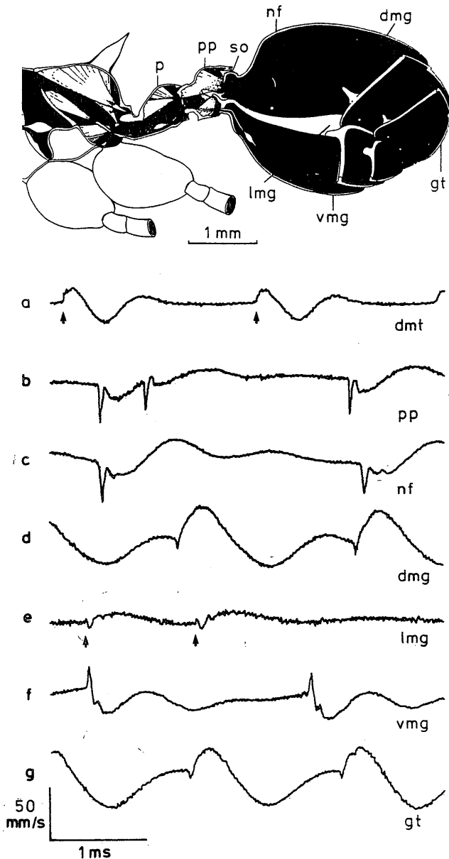
Fig. 1. Drawing of the abdomen and part of the thorax of a leaf cutting ant (modified from Markl (1968)) with typical stridulatory velocity waveforms recorded by LDV at different points on the ant. dmG dorsal mid-gaster; dmT dorsal mid-thorax (not shown in drawing); gt gaster tip; lmg lateral mid-gaster; nf near file on gaster; p petiole; pp postpetiole; so stridulatory organ; vmG ventral mid-gaster. Arrows in a and e mark the tooth strikes
