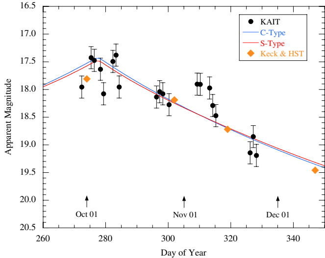
Figure 3. R -band photometry from KAIT (black circles) and from Keck and HST (orange diamonds) within a 6'' radius circular aperture as a function of Day of Year in 2013. Lines show the brightness variation expected of an asteroid following the inverse square law of distance and with phase functions appropriate for C-type (blue) and S-type (red) surfaces.
