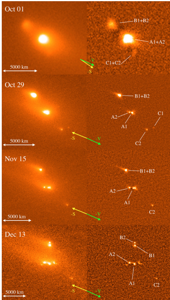
Figure 1. Four epochs of R3 imaging from 2013 (cf. Table 1) shown as raw images (left column) and spatially filtered to suppress diffuse coma (right column). October 1 data are from Keck, all the rest from HST . Each panel has north to the top, east to the left, and has dimensions 14'' \times 12'' . The projected anti-solar direction is shown by a yellow arrow marked “-S.” Projected negative velocity vector is indicated by a green arrow marked “-V.” Components discussed in the text are identified.
