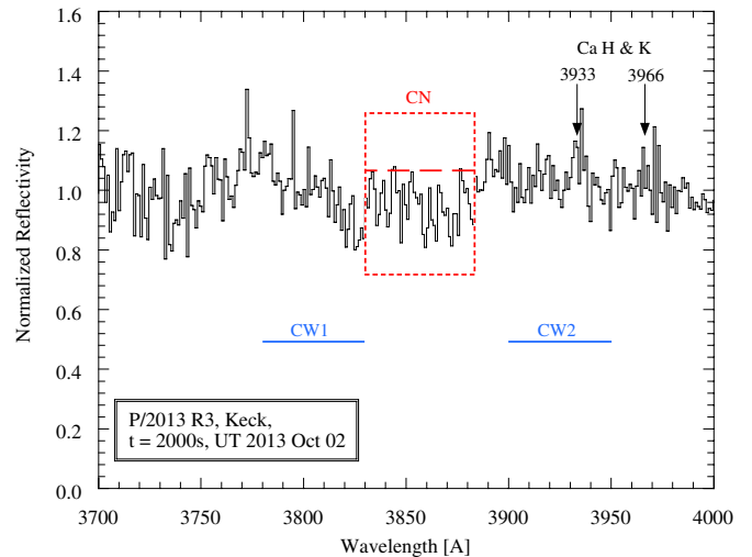
Figure 2. Normalized reflection spectrum in the vicinity of the CN band (outlined in red dashed box). Blue lines marked CW1 and CW2 denote regions of the spectrum used for continuum assessment. The 5σ limit to CN emission is marked with a horizontal long-dashed line. Residual H and K lines of calcium are marked.
